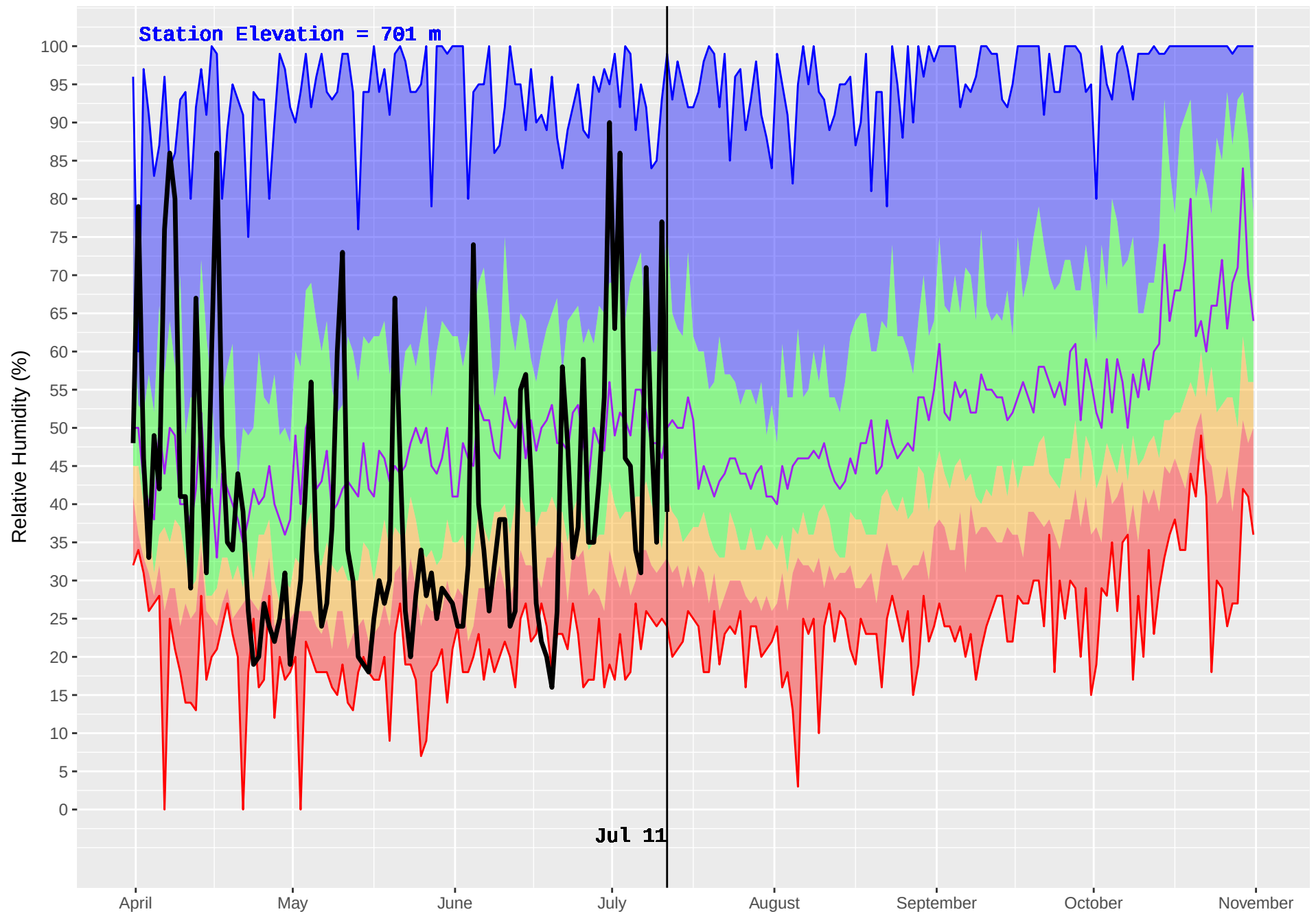
HORSEFLY (230) : Historical (1971–2016) and Current (2018) Noon Relative Humidity
