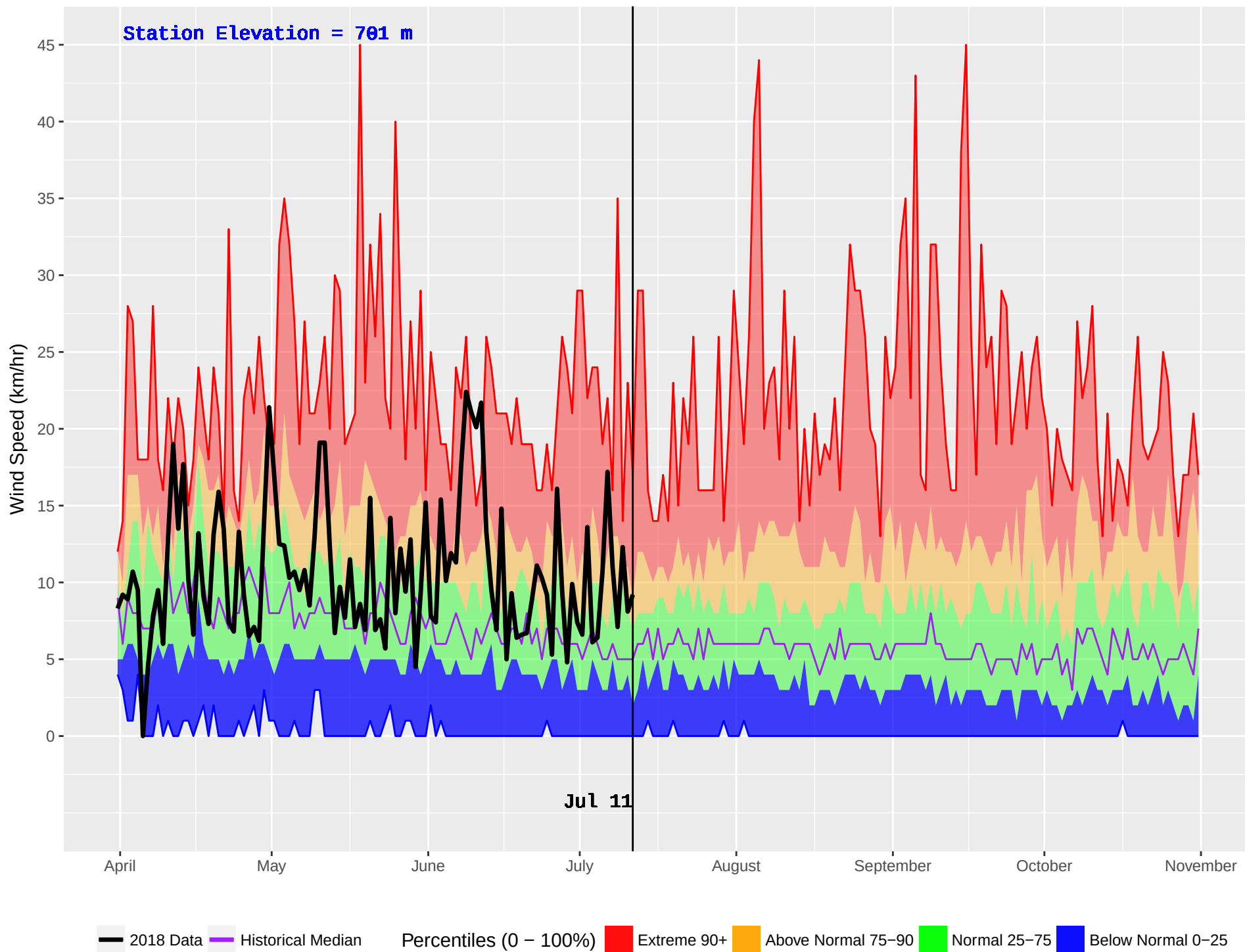
HORSEFLY (230) : Historical (1971–2016) and Current (2018) Noon Wind Speed
