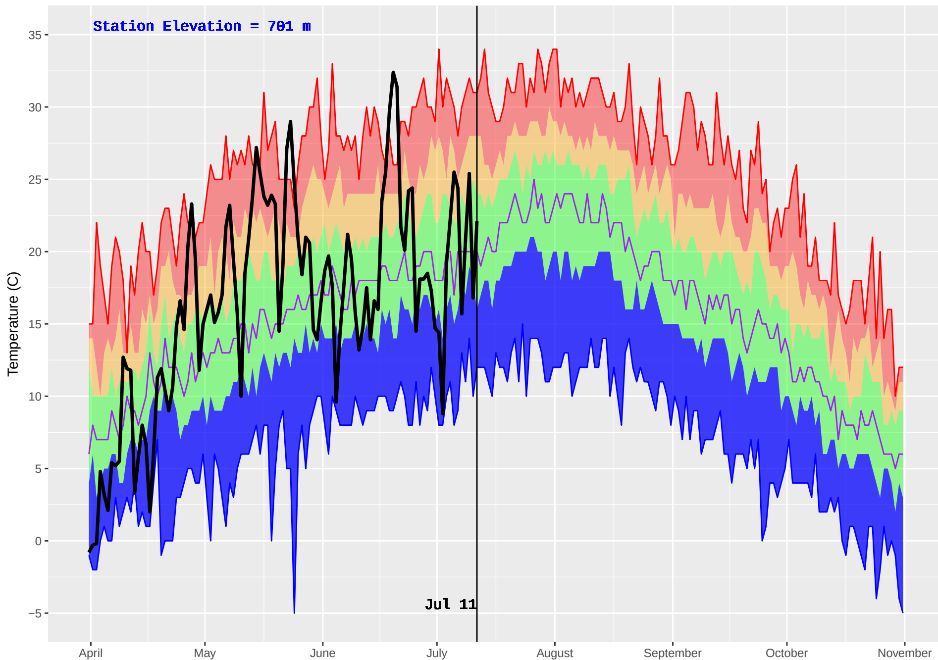
HORSEFLY (230) : Historical (1971–2016) and Current (2018) Noon Temperature
